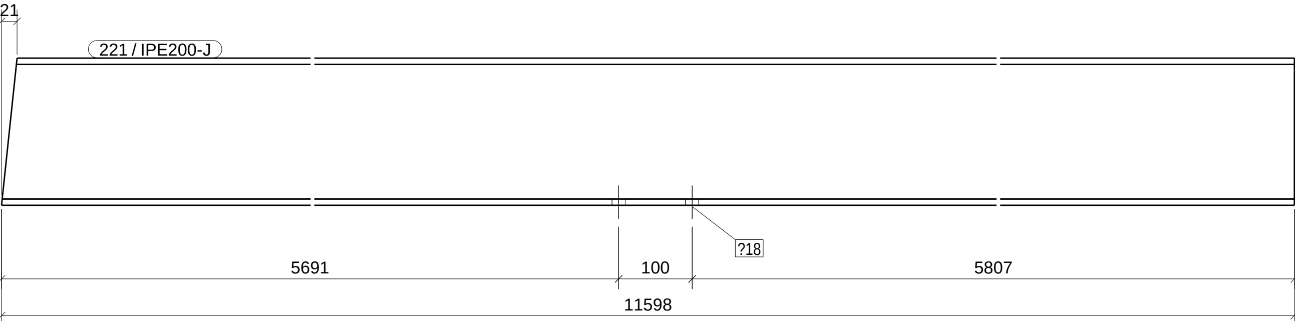
FRONT VIEW
